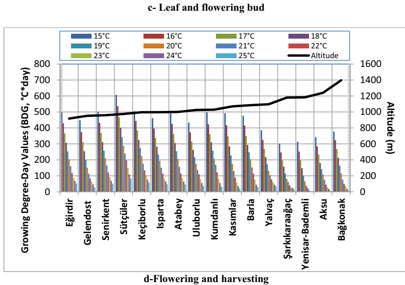
Figure 1. Relationship between GDD values and altitude in different phenological periods of oil rose plant
