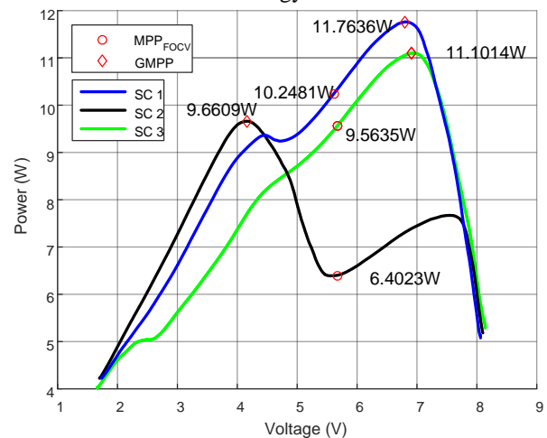
Figure 9. MPP and GMPP values for FOCV method
